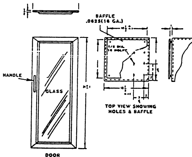
Figure L-1 - Vertical flame resistance textile apparatus. All given dimensions are in inches. System International (S.I.) unit: 1 inch = 2.54 cm.
